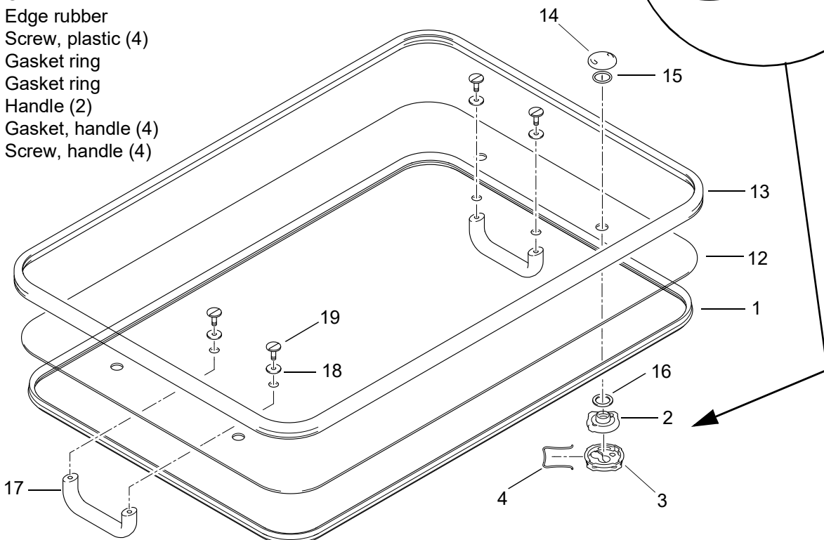
Fig. 802 Eleon hatches - Components (part 2)
