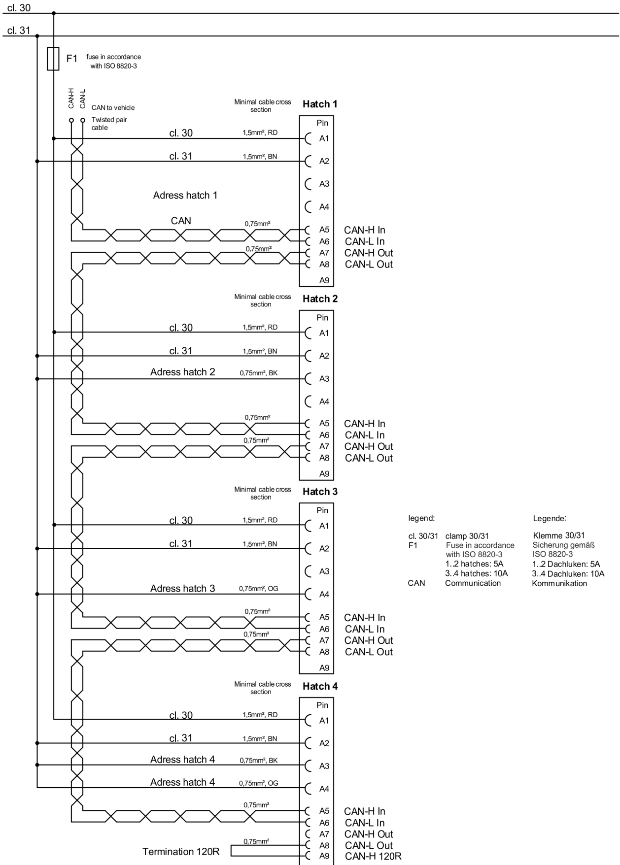
Fig. 601 Wiring diagram 1..4 roof hatches via CAN bus
