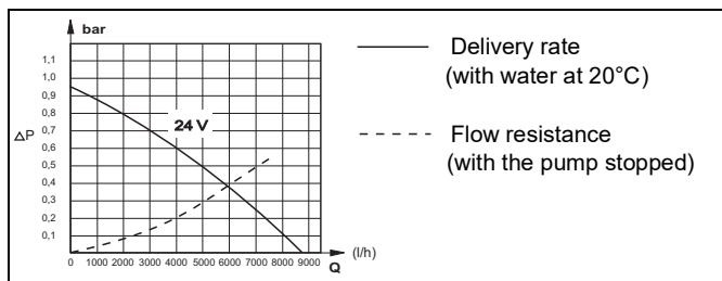
Fig. 14: Delivery rate and flow resistance U 4855 circulating pump
