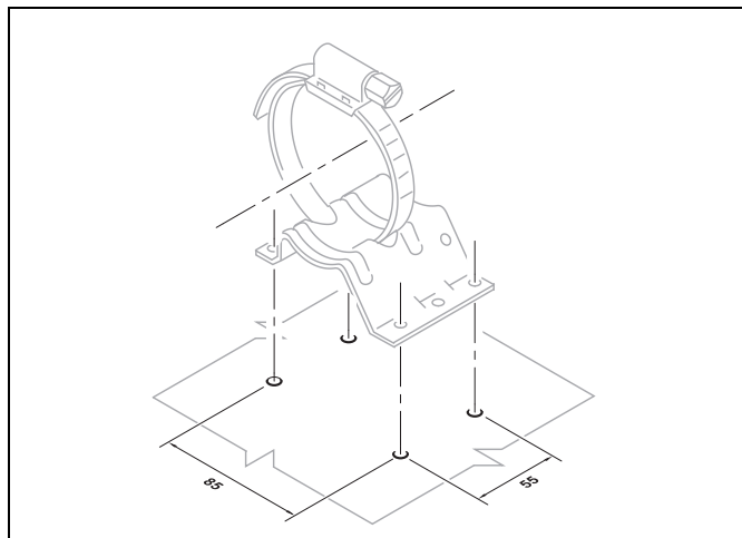
Fig. 13: Hole pattern for the stand for U 4855 circulating pump
