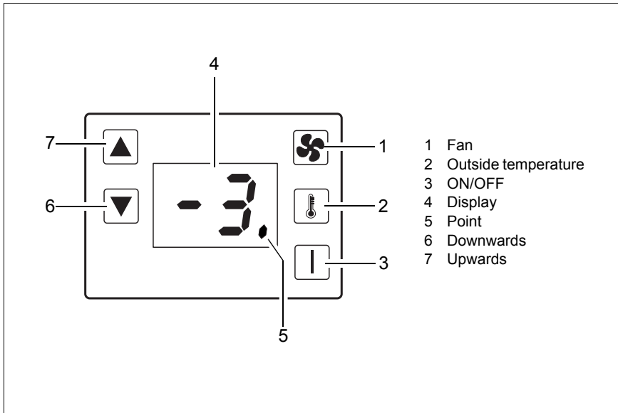
Fig. 1: Control panel
